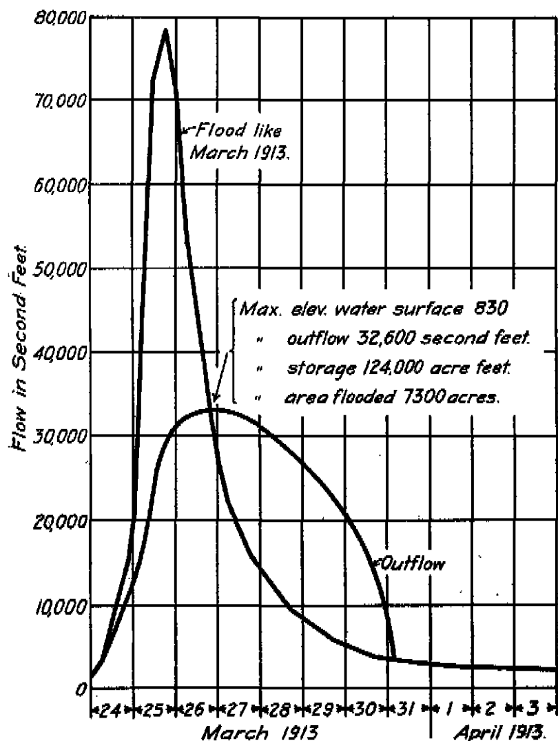
Fig. 40.—Hydrographs showing size of Flood of March, 1913, at Huffman Retarding Basin, as compared with the rate of outflow from the Basin if it had been in existence.
