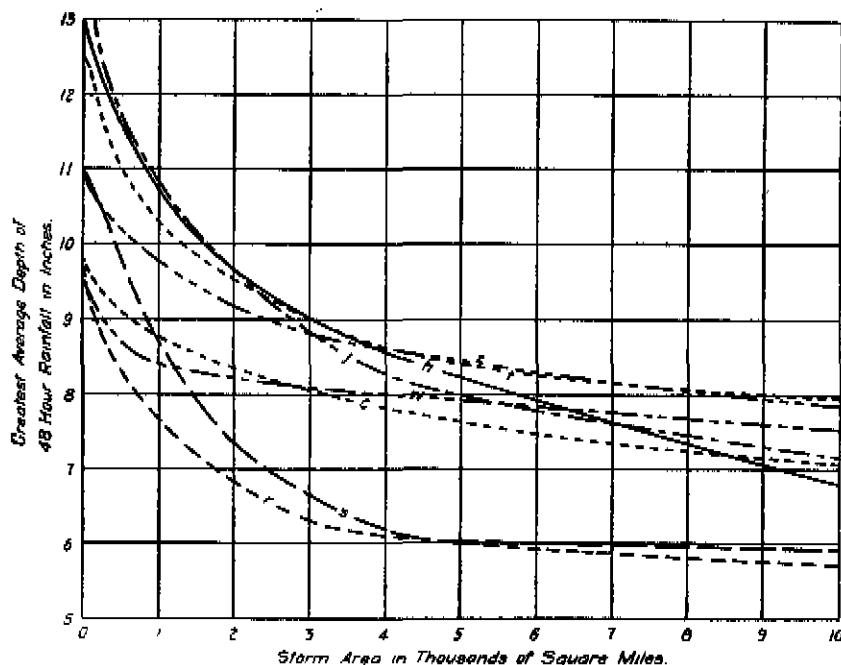
Fig. 28.—Maximum 48-Hour Rainfall for the Greatest Recorded Storms in the Upper Mississippi Valley. The diagram shows the average depth of 48-hour rainfall in inches over different sized areas in the center of each storm.
