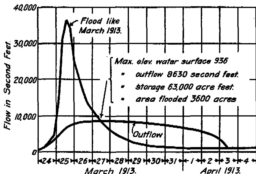
Fig. 38.—Hydrographs showing size of Flood of March, 1913, at Lockington Retarding Basin, as compared with the rate of outflow from the Basin if it had been in existence.
