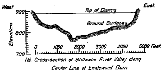
Fig. 33.—(a) Cross section of Englewood dam; (b) Cross section of Stillwater River Valley along the center line of the Englewood dam. These cross sections are typical of the conditions found at the various dam sites.
