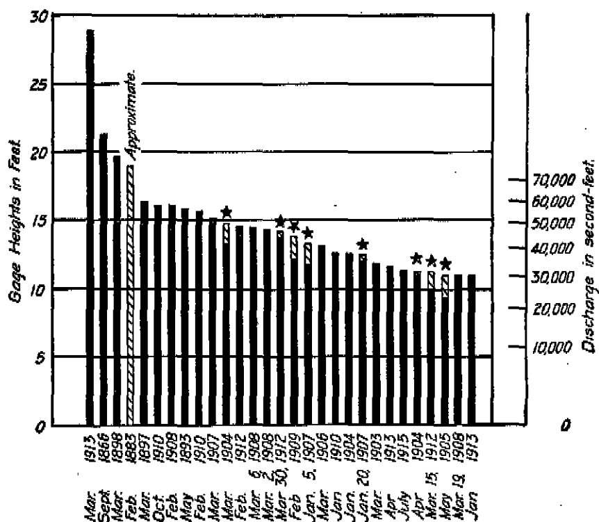
Fig. 21.—Maximum Miami River Stages of 11 feet and above, at Dayton, Ohio. Based upon daily gage readings of U. S. Weather Bureau from Dec. 22, 1892, to Jan. 1, 1916, and fragmentary early records. Crest stages marked with star are estimated from hydrographs.
