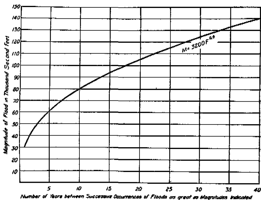
Fig. 23.—Curve showing Frequency of Floods at Dayton, Ohio. Based on the records shown in Fig. 21. The horizontal scale shows the probable average number of years which will elapse between successive occurrences of floods equalling or exceeding any given size as shown on the vertical scale.
