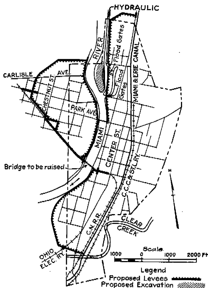
Fig. 49.—Map of Franklin, Ohio, showing proposed local flood protection.
