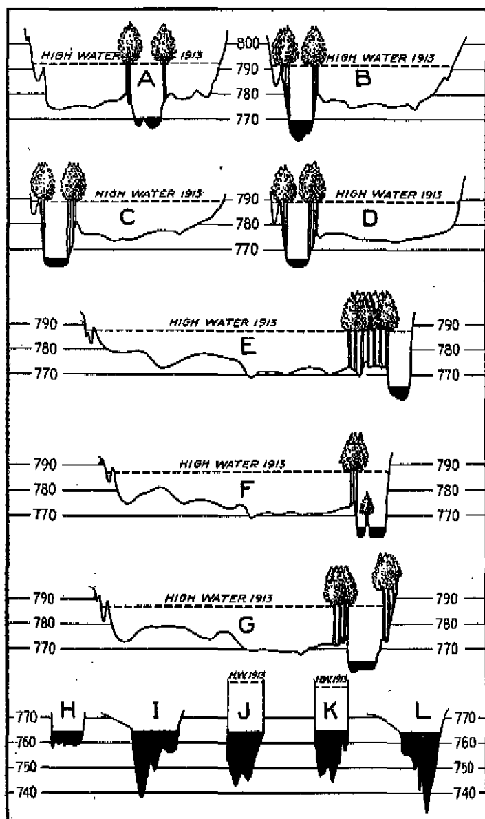
Fig. 24.—Cross Sections of the Miami Valley near Tadmör, Ohio, used in calculating the maximum discharge rate during the flood of March, 1913. The relative position of the various cross sections is shown in the plat, Fig. 25. Each cross section shows the elevation of the cultivated fields across the valley floor, the high water line, the position of the trees along the river banks, and the low water cross section of the river channel (indicated in solid black) at the time the measurements were taken in June, 1913. The scour in the bed of the river channel caused by the contraction at the canal aqueduct crossing is shown in cross sections H, I, J, K, and L.
