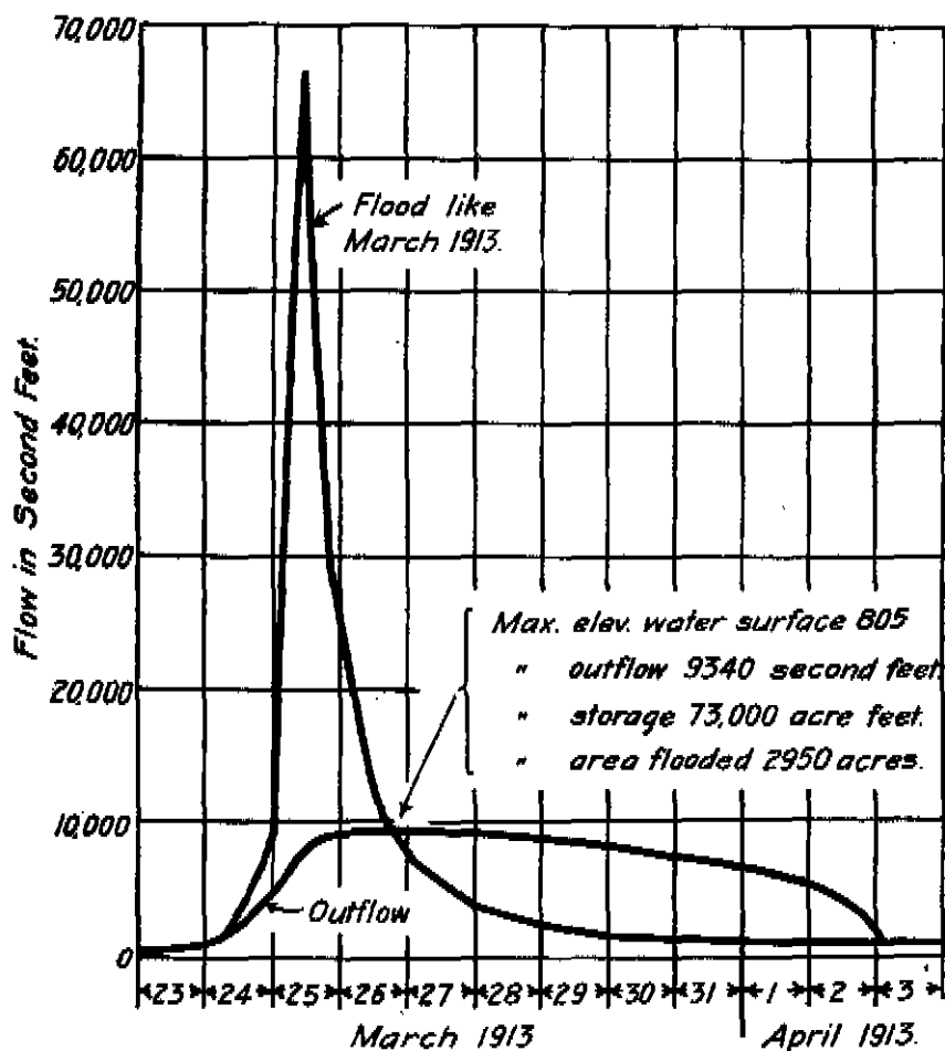
Fig. 36.—Hydrographs showing size of Flood of March, 1913, at German-town Retarding Basin, as compared with the rate of outflow from the Basin if it had been in existence.
