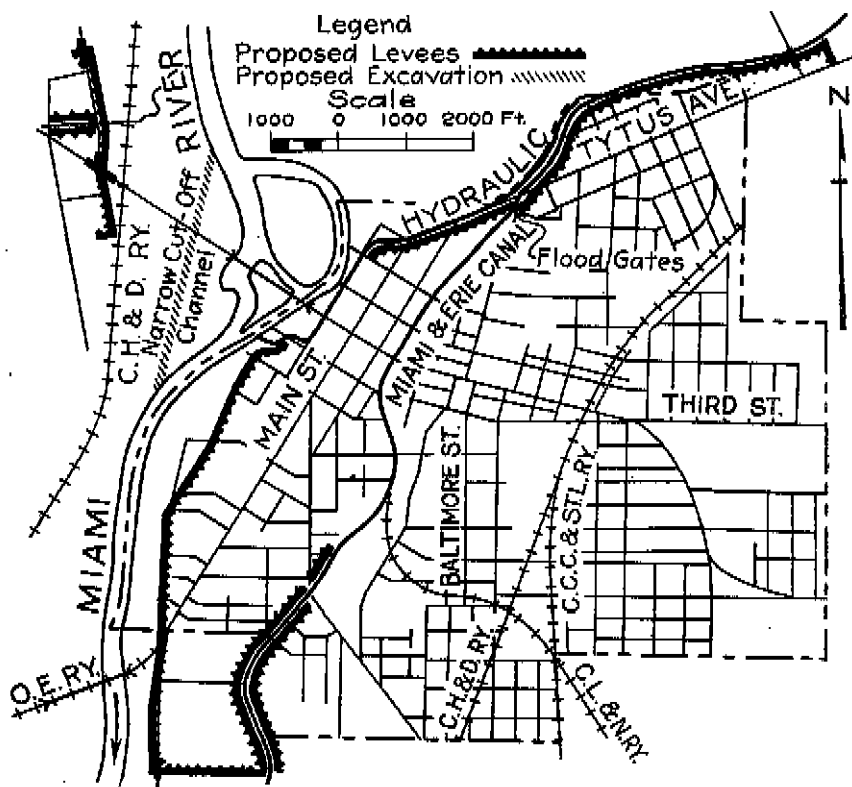
Fig. 50.—Map of Middletown, Ohio, showing proposed local flood protection.
