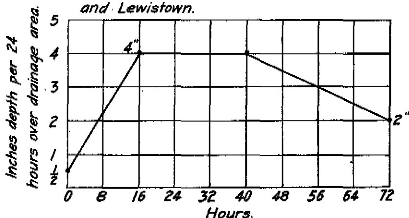
Fig. 30.—Maximum Flood Runoff Curves adopted for use in designing the Miami Valley Retarding Basins and Outlet Conduits.
