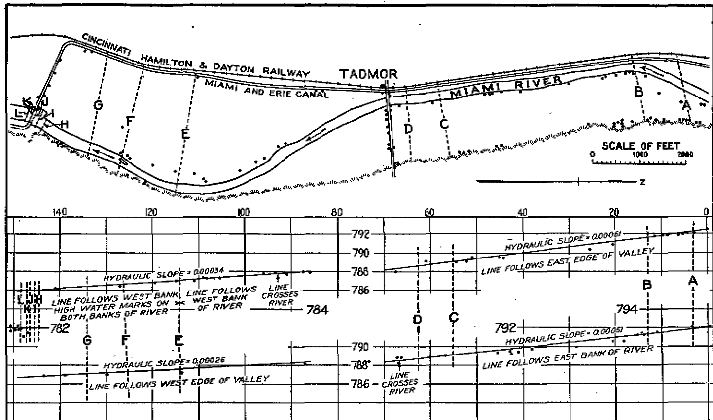
Fig. 25.—Plat of Miami Valley near Tadmor, Ohio, and Maximum High Water Profile, during flood of March, 1913, showing locations of measured cross sections of the valley and the points, indicated by round dots, where high water elevations were measured. The cross sections indicated by letters are shown in Fig. 24. The profile shows the sudden drop of about 4 feet in the water surface in passing through the contracted opening caused by the aqueduct crossing of the Miami and Erie Canal.
