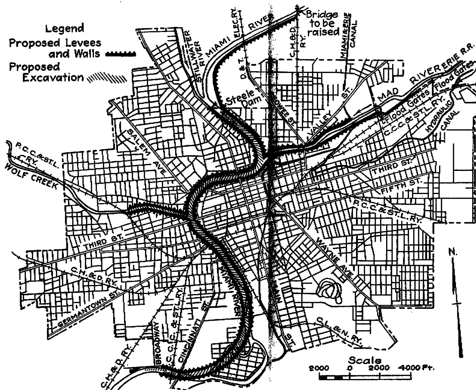
Fig. 45.—Map of Dayton, Ohio, showing proposed local flood protection.
