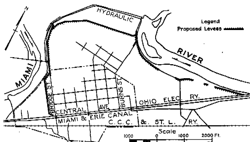
Fig. 46.—Map of West Carrollton, Ohio, showing proposed local flood protection.
