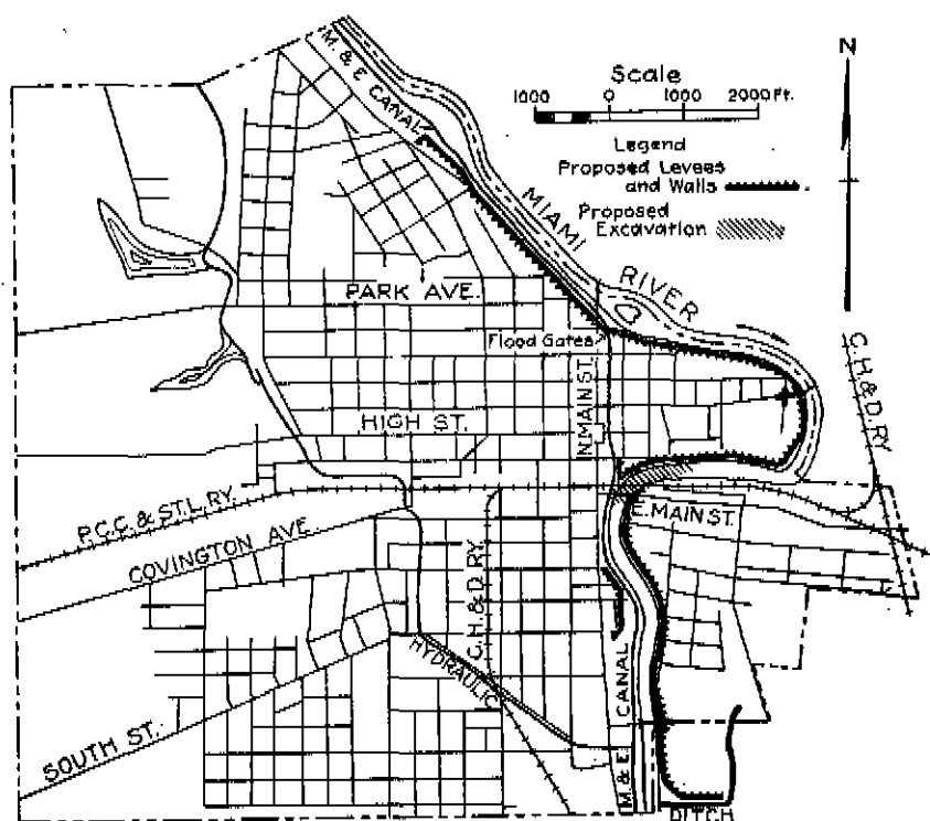
Fig. 43.—Map of Piqua, Ohio, showing proposed local flood protection.
