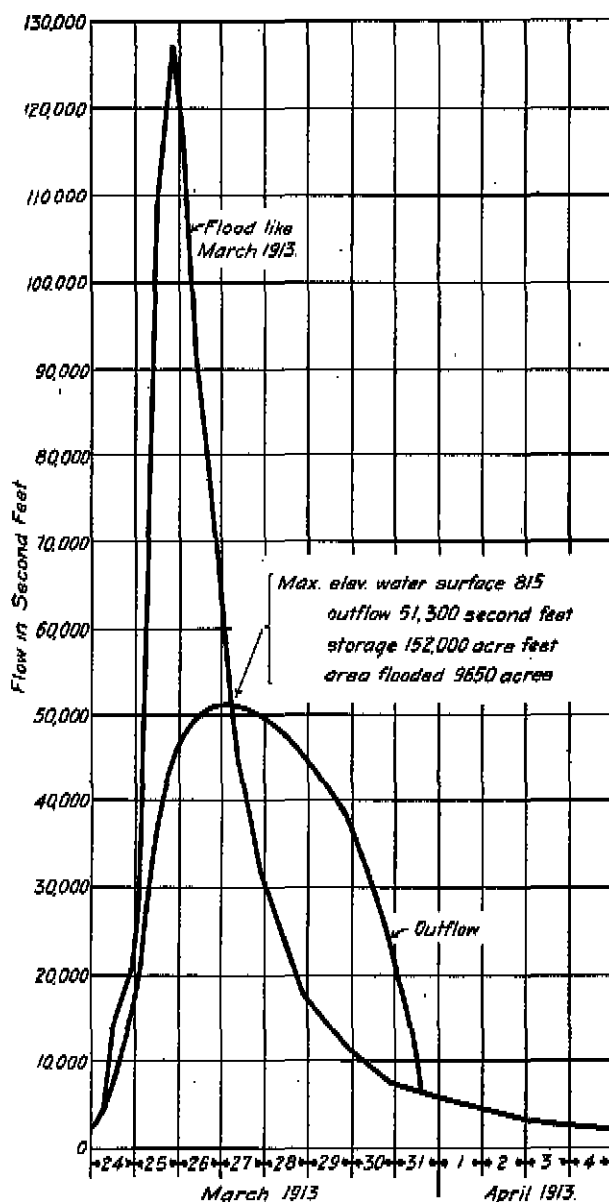
Fig. 39.—Hydrographs showing size of Flood of March, 1913, at Taylorsville Retarding Basin, as compared with the rate of outflow from the Basin if it had been in existence.
