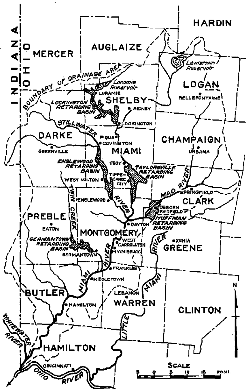
Fig. 1.—Map of Miami River drainage area showing location of proposed retarding basins.
