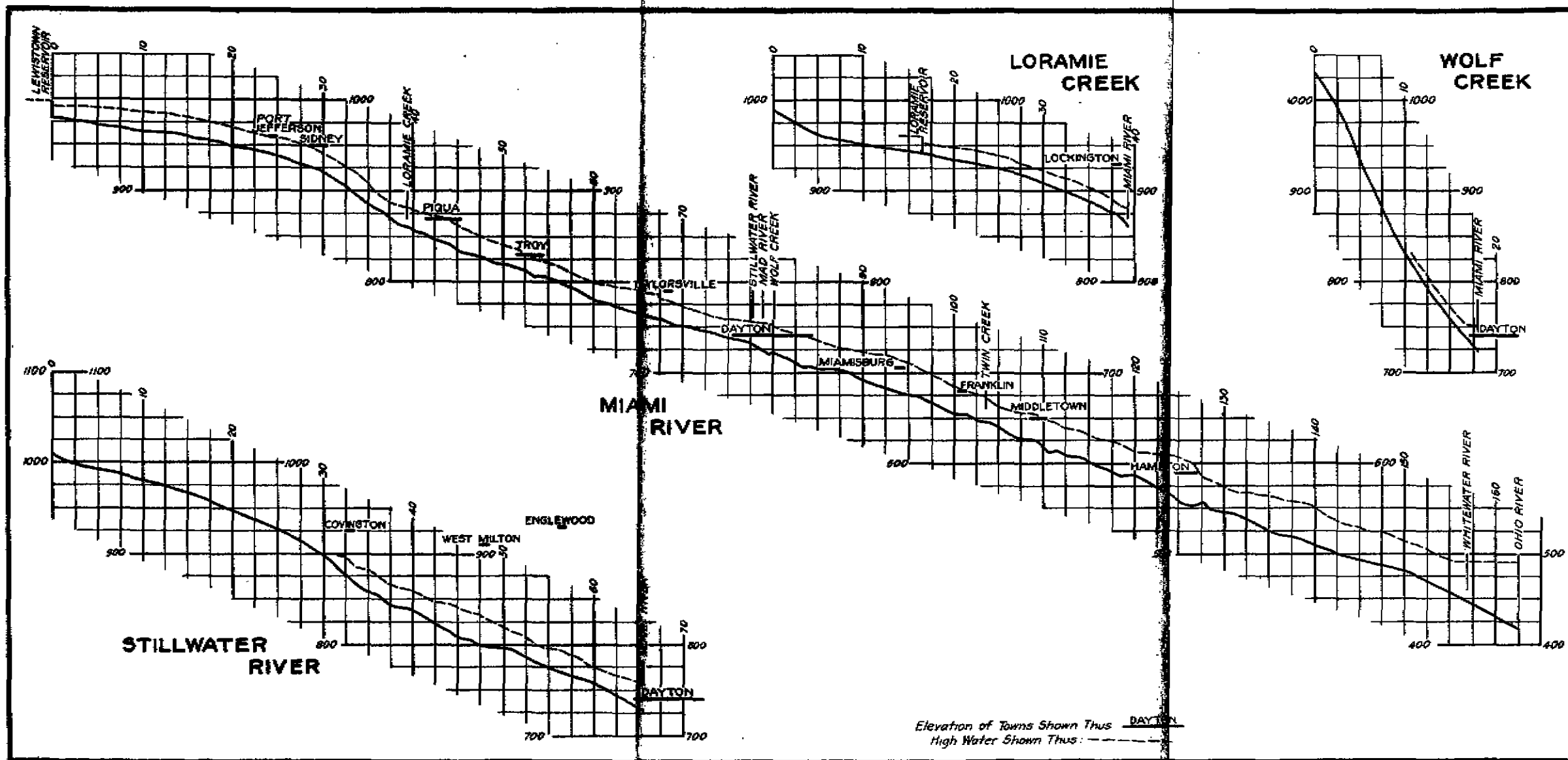
Fig. 11.—Condensed Profiles of Miami River, Stillwater River, Loramie Creek, and Wolf Creek, showing high water line of March, 1913. Horizontal distances are in miles, vertical distances in feet.
