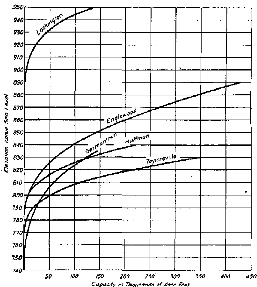
Fig. 32.—Capacity Curves for all of the Proposed Retarding Basins, showing the capacity of each basin in acre feet for all depths of water.
