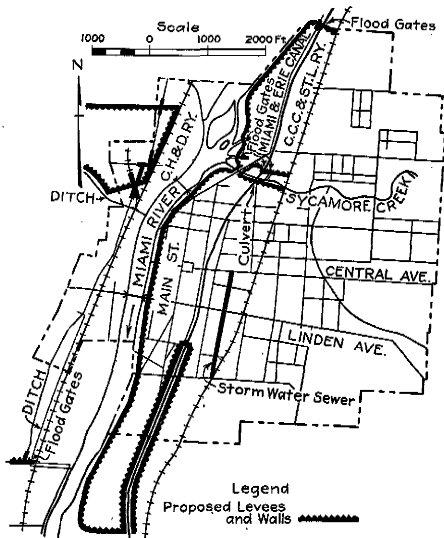
Fig. 47.—Map of Miamisburg, Ohio, showing proposed local flood protection.
