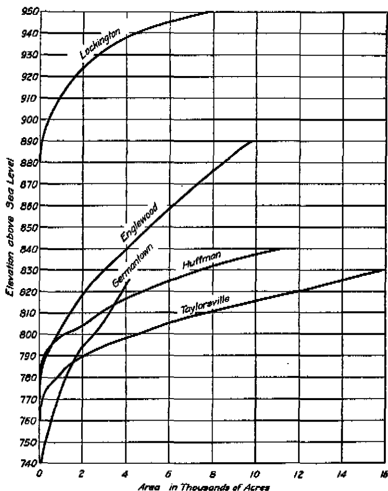
Fig. 31.—Area Curves for all of the Proposed Retarding Basins, showing the area of the water surface in acres for all depths of water.
