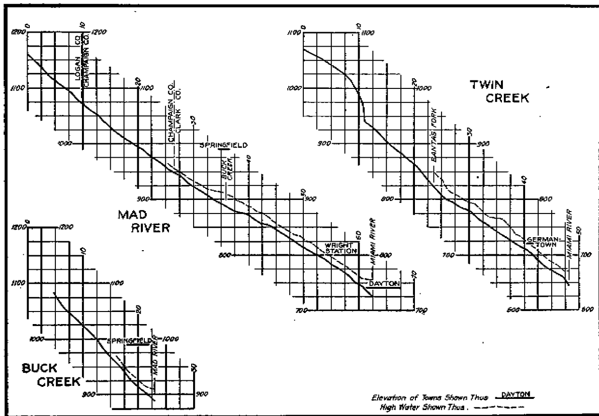
Fig. 10.—Condensed Profiles of Mad River, Buck Creek, and Twin Creek, showing high water line of March, 1913. Horizontal distances are in miles, vertical distances in feet.
